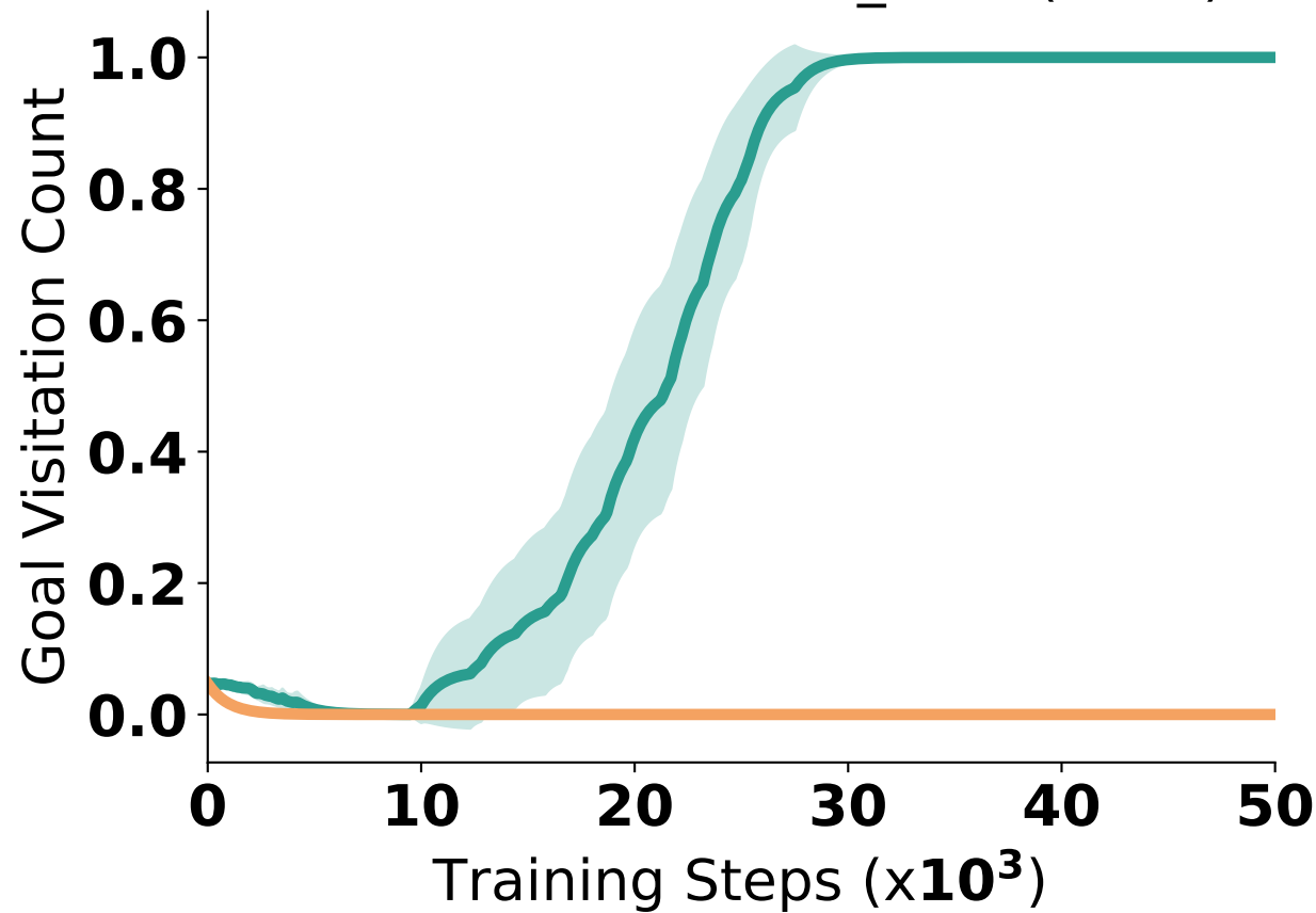
Gridworld-Bottleneck_Level(5.0%)
